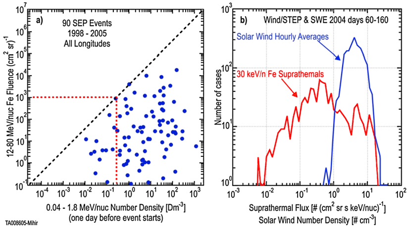
Fig. 5 Left: Fluence of >12 MeV/nuc Fe in large SEP events vs. suprathermal Fe density one day prior to the onset of the corresponding SEP event (after Mewaldt et al. 2012b). Right: Hourly averaged intensity of suprathermal \sim 30 keV/nuc Fe (red) and number density of solar wind Fe (blue) for a 100 day period in 2004 (taken from Mason et al. 2005)
