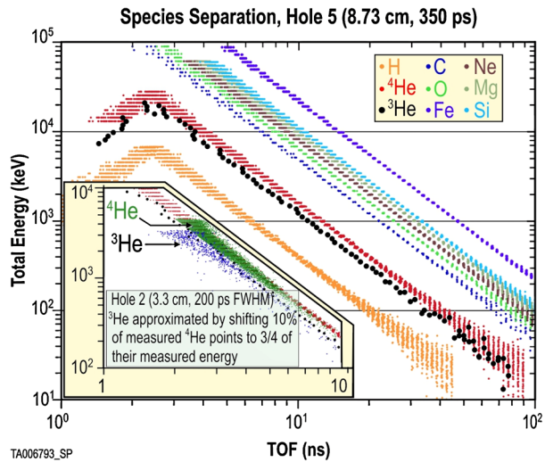
Fig. 21 Representative species separation for EPI-Lo holes 2 (22.5° from the instrument normal) and 5 (the holes about the instrument perimeter, 90° from instrument normal) based on measured TOF resolution performance on test model. Data taken using an alpha source in hole 2 is overlaid on the hole 2 simulated data. ^3\text{He} is well distinguished from ^4\text{He} at 1:100 abundance ratio to \geq 1.5 MeV/nuc. The best performance for species identification is in the 64 holes at the 3, 4 and 5 positions, at 45°, 67.5°, and 90° from the instrument normal
