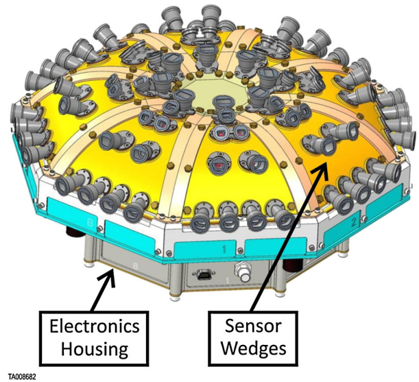
Fig. 15 EPI-Lo mechanical design
