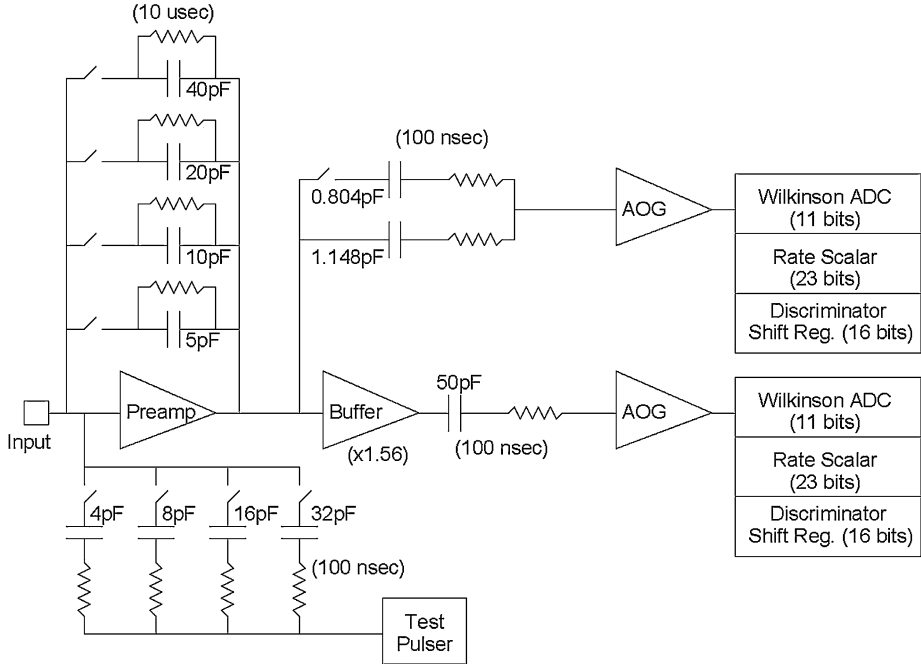
Fig. 37 Schematic diagram of one PHASIC channel
