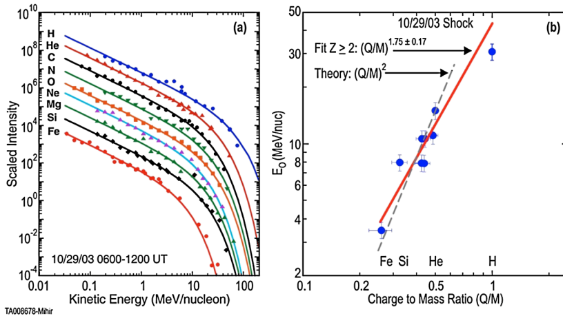
Fig. 9 Heavy ion energy spectra in a CME-associated SEP event are fitted with Ellison and Ramaty (1985) spectral form for differential intensity j = j_0 E^{-\gamma} \exp(-E/E_0) . All elements have the same spectral index of \gamma = 1.3 (Mewaldt et al. 2005). Spectra of different elements are offset for clarity. (Right): Values of the e-folding energies E_0 versus the ion's Q/M ratio. Fits to the values of E_0 yield a (Q/M)^{1.75} dependence, which according to Li et al. (2009) is appropriate for a strong quasi-parallel shock
