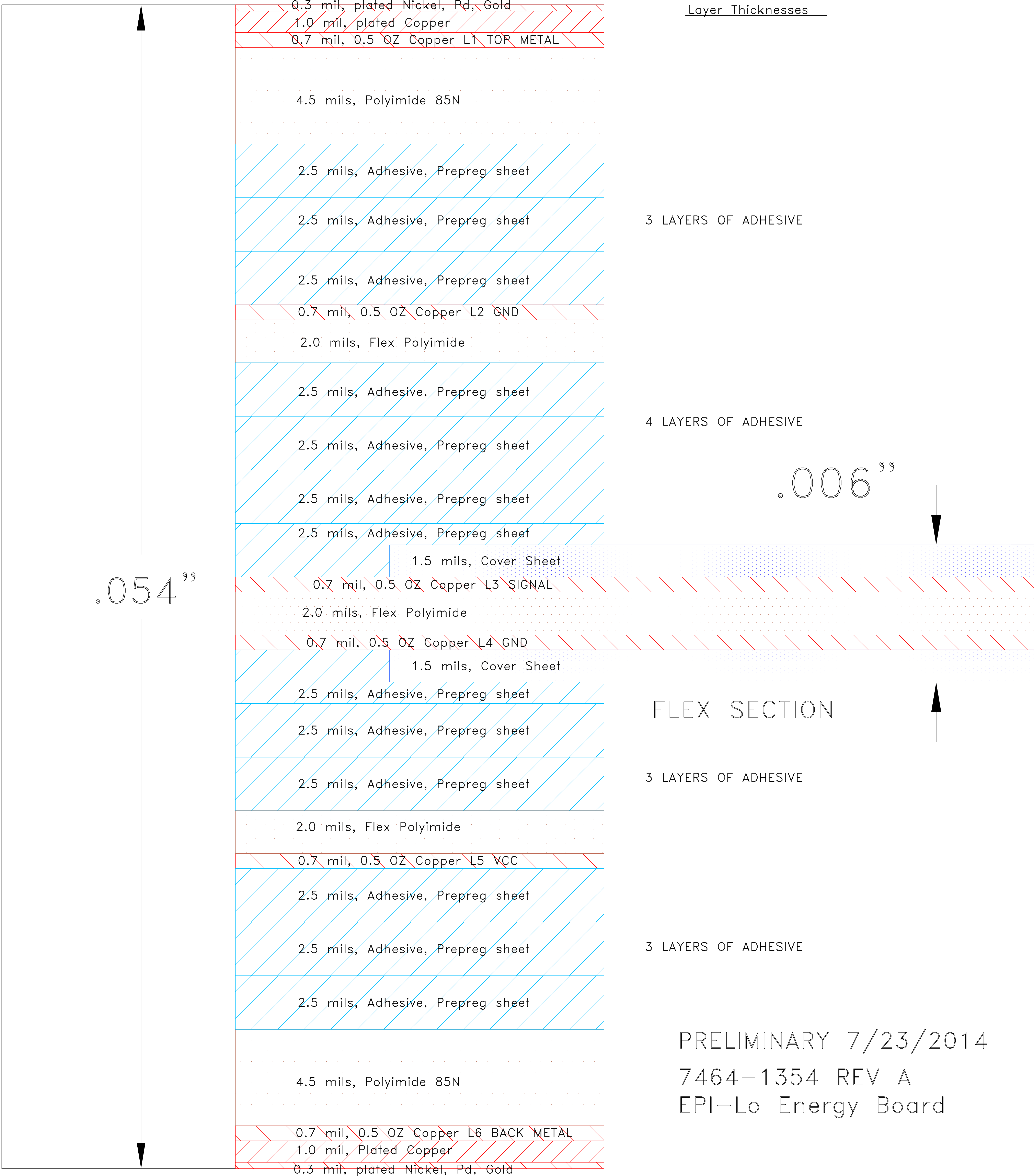
STACK-UP OF THE RIGID AND FLEXIBLE LAYERS
